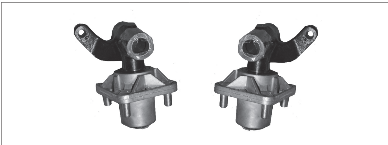
70673G03 LEFT HAND SPINDLE ASSEMBLY 2001+ TXT; 2017+ TXT ELITE; 2017+ 72V TXT
