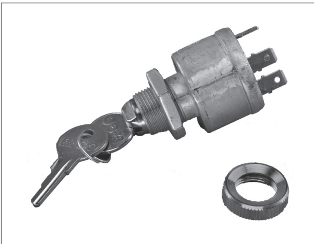
33639G01 STANDARD IGNITION SWITCH W/ LIGHTS 1996+ TXT
