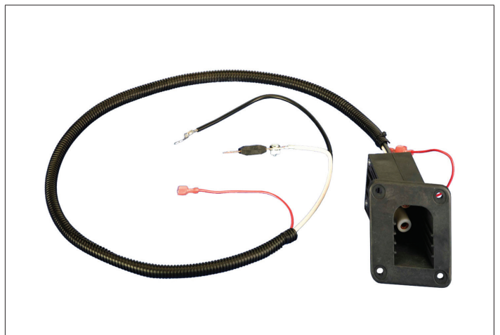
73063G01 36V CHARGER RECEPTACLE W/ HARNESS 1996-2011 TXT
