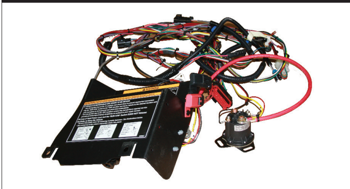
618955 ELECTRIC HARNESS ASSEMBLY W/ HD SOLENOID 2009+ RXV
