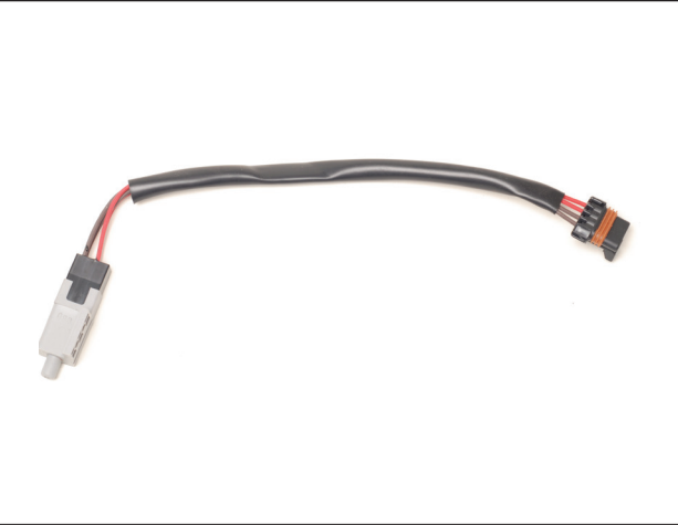
607605 BRAKE AND ACCELERATOR PEDAL SWITCH 2008+ RXV; 2017+ RXV ELITE
